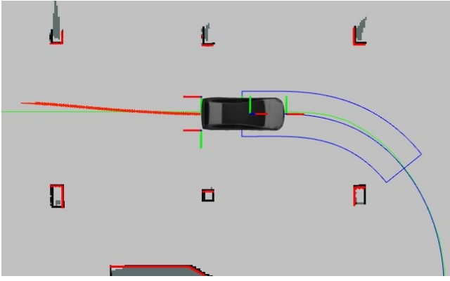
Fig. 8. Software stack running in Drake: Grey map in background, red arrow line visualizes odometry messages over time, red points on obstacles are the LiDAR output, the blue line is the control path from the pure-pursuit controller, the curved blue rectangle is the DVB and the green line the predefined path.
