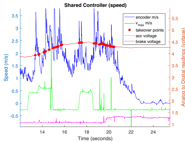
Fig. 13. Shared controller applied to speed: The red line shows the DVB advised speed for the current path. The blue line is the encoder speed measurement. Every takeover point is marked with a red dot. When the human is pressing the accelerator pedal the green line increases likewise the magenta line when the brake pedal is pressed.
