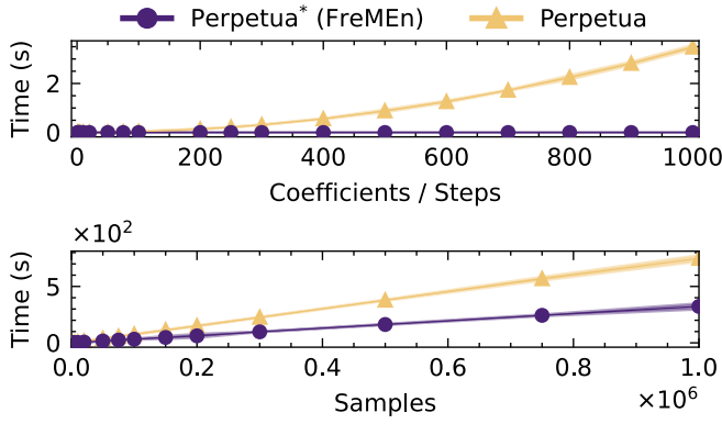
Fig. 9. Computational Complexity: prediction (top) and update (bottom) steps for Perpetua* with a FreMEN prior versus Perpetua . Top: prediction time as a function of Fourier coefficients in Perpetua* and simulation steps in Perpetua . Bottom: update time with up to 1 million samples. Results are averaged over five random seeds. Perpetua* exhibits faster computation in both cases by replacing Perpetua ’s state machine with our Bayesian model selection mechanism.
