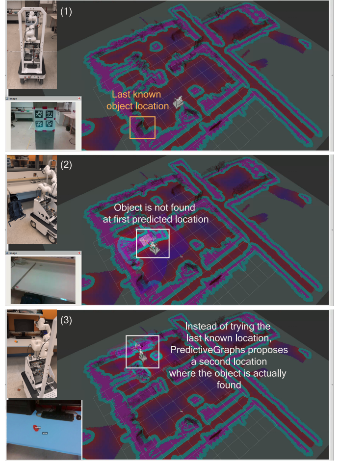
Fig. 15. Qualitative Navigation Result in Real-World - Replanning: Open-vocabulary query “Could you get me a healthy vegetable?” with query time 29 hours after the last map update. (1) PredictiveGraphs identifies the target object as a carrot. (2) PredictiveGraphs proposes an initial candidate location; however, upon navigating to it, the object is not found. (3) Instead of reverting to the object’s last known location, PredictiveGraphs predicts a new location where the carrot is successfully found, highlighting the robustness of our tempo-spatio-semantic scene graph in dynamic scenes.
