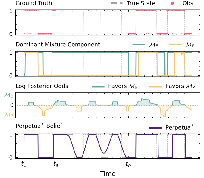
Fig. 10. Illustrative Example Perpetua* : An object undergoes semi-static changes at varying rates (top row). We maintain a mixture of persistence and emergence filters (each comprising three components in this example) that adapt their belief as new observations arrive. The second row shows the dominant component of the persistence and emergence filters (see (6)) at each time step. As time progresses, our Bayesian model selection criterion (see (8)) identifies the mixture that best explains the observed data (third row). Notably, between times t_a and t_b , where no observations are available, the log posterior odds keep evolving due to our switching prior, whereas the dominant mixture component remains frozen. The bottom row shows the final Perpetua* prediction, obtained by mixing the output of both mixture models at each time step, as shown in (9). By leveraging the switching prior (cf. Fig. 2 and Fig. 4), Perpetua* maintains accurate predictions even in the absence of observations.
