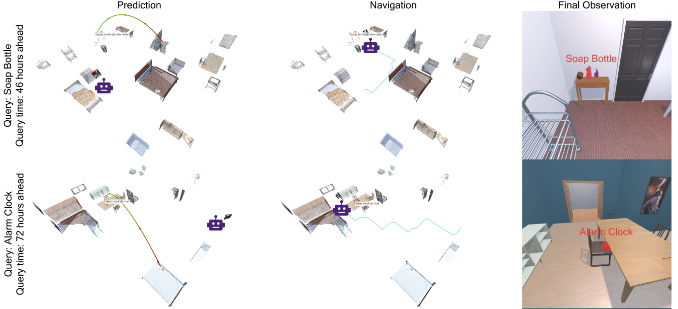
Fig. 13. Qualitative Navigation Results in ProcTHOR: The top row shows a navigation sequence where PredictiveGraphs is queried 46 hours after the last map update (top-down map shown in the first row, third column of Fig. 16). In the first column, our method predicts that the soap bottle has moved from the dresser (red spline tip) to a side table (green spline tip). The second column shows the robot navigating to the predicted location, with its path marked in blue. The final column displays the successful detection of the soap bottle. The bottom row depicts a similar example with an alarm clock queried 72 hours after the last map update (top-down map shown in the third row, first column of Fig. 16).
