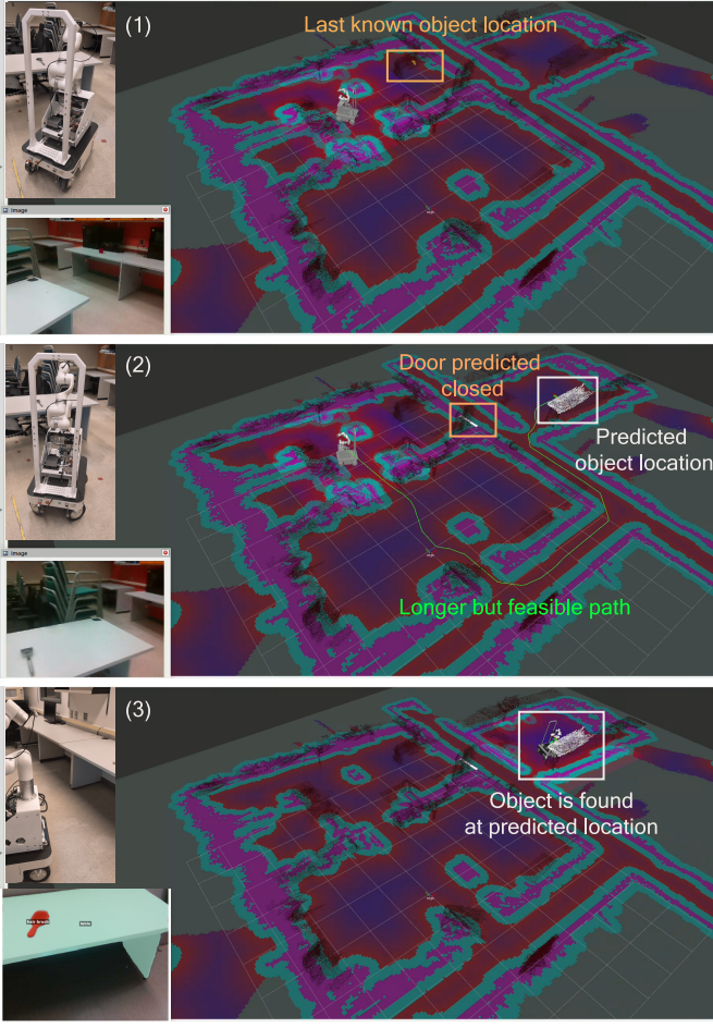
Fig. 14. Qualitative Navigation Result in Real-World - Topological Graph Change: Extended version of Fig. 7. The open-vocabulary query is “Is there something useful to comb my hair?”, with query time 146 hours after the last map update. (1) Shows the last known position of the relevant object identified by PredictiveGraphs (a hair brush). (2) Our method predicts that the hair brush is in another room and detects that the door along the shortest path is closed; this updates the cost map, prompting the planner to generate a longer but feasible path. (3) The agent successfully locates the target object.
